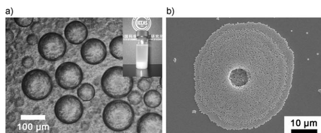
Figure 2. a) Optical microscope image of the W/O Pickering emulsion stabilized by CMPTS-modified \text{SiO}_2 colloids (inset: the emulsion appearance); b) SEM image of one emulsion drop after drying.
